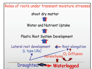
Fig. 2. Contribution of root plasticity
