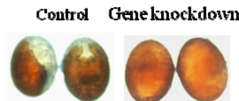
Fig. 4. Legumains are critically needed for tick embryogenesis
